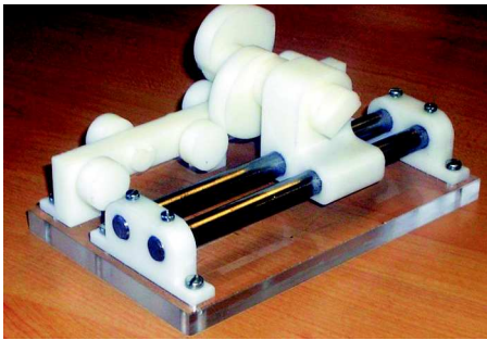
Figure 14: Layout of the two coaxial conjugate-cam mechanism on the same shaft
