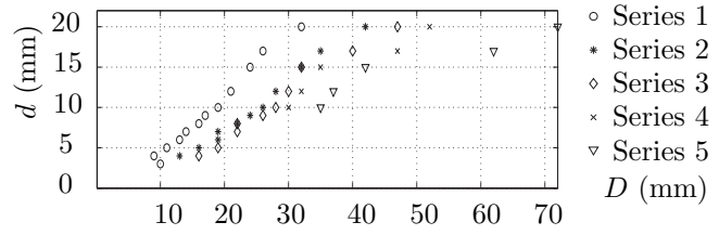
Figure 13: Dimensions of the SKF bearings
