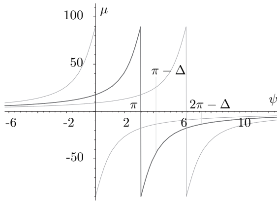
Figure 7: Pressure angle distribution
