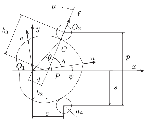
Figure 3: Parameterization of Slide-o-Cam
