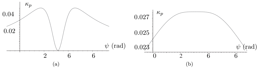
Figure 10: Pitch-curve curvature for p = 50 mm: (a) \eta = 1/\pi and (b) \eta = 2/\pi
