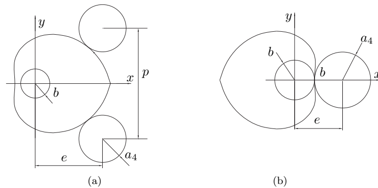
Figure 6: Constraints on the radius of the roller: (a) a_4/p < 1/2 ; and (b) a_4/p \leq \eta - b/p .
