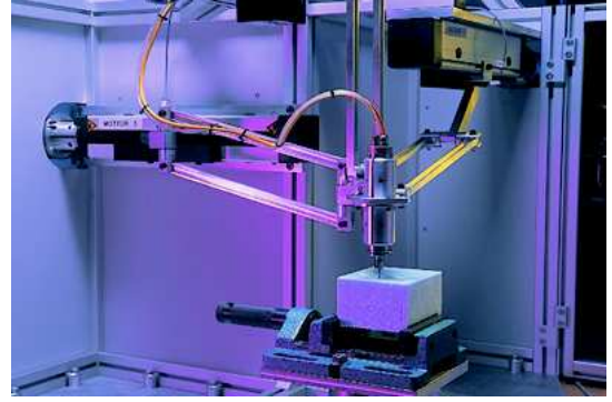
Figure 2: The Orthoglide
