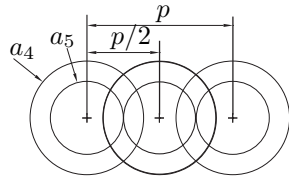
Figure 12: Geometric constraint on the roller-pin radius
