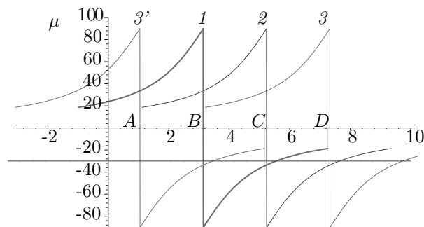
Figure 17: Pressure angle for the three cams
