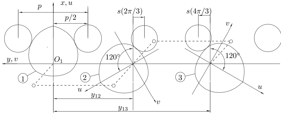
Figure 16: Layout of the non-coaxial conjugate-cam mechanism on three parallel shafts
