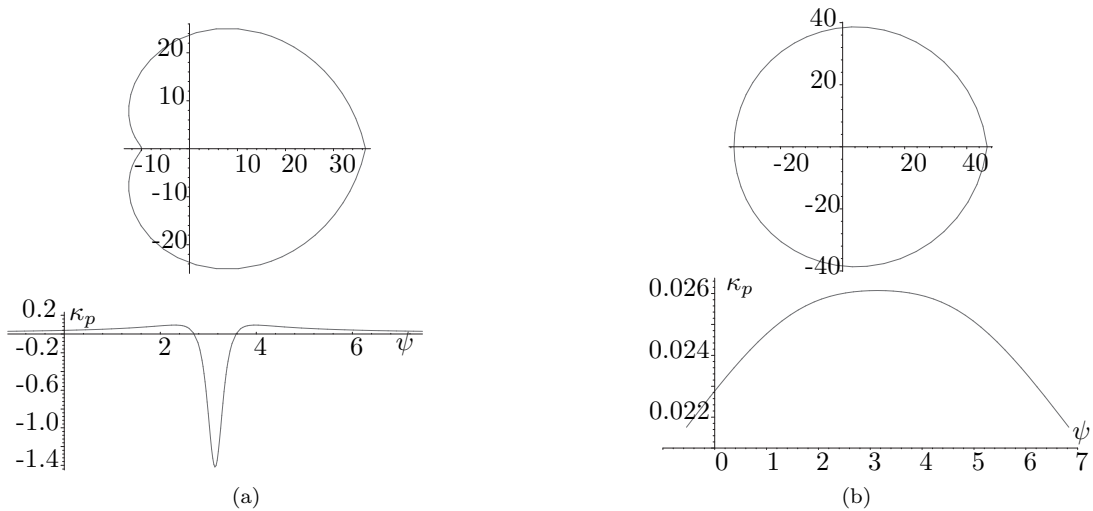
Figure 9: Pitch-curve profiles and their corresponding curvatures with p = 50 mm:
