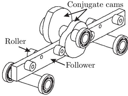
Figure 1: Layout of Slide-o-Cam
