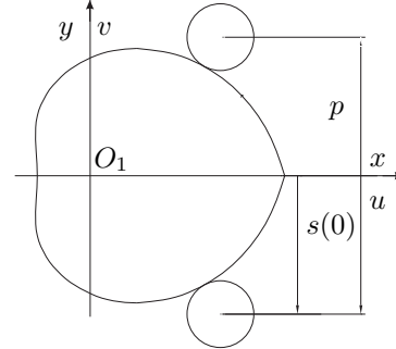
Figure 4: Home configuration of the mechanism
