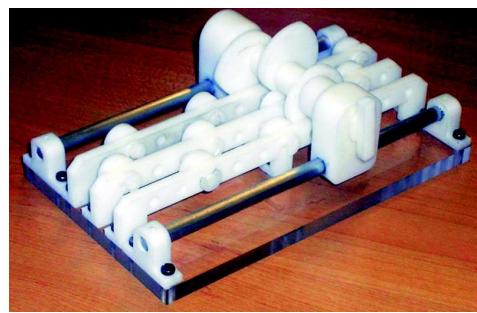
Figure 15: Layout of the three conjugate-cam mechanism on the same shaft
