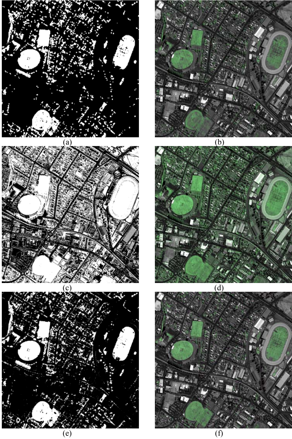
Fig. 3. The vegetation map and extraction of set 2: (a) VTC' map map, (b) extraction using VTC' map, (c) VI map, (d) extraction using VI, (e) HRNDVI map, (f) extraction using HRNDVI.
