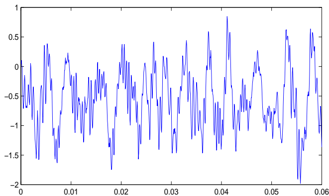
Figure 3: A discretized path (X(\Delta_N), \dots, X(N\Delta_N)) with \underline{H} = 0.3 and \tau = 2
