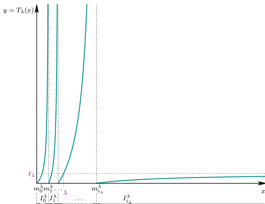
FIGURE 1. Top: Graphs of the homographic functions h_i . Bottom: Graph of the transformation T_\lambda . (Here \lambda = 1.5 )
