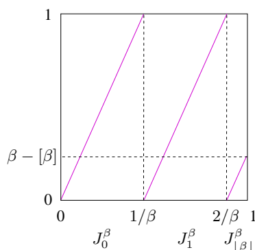
FIGURE 5. Graph of S_\beta for \beta = 9/4 .
