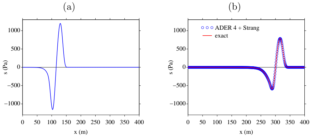
Figure 4: test 1, homogeneous viscoelastic medium. Stress \sigma at the initial instant (a) and after 200 time steps (b).
