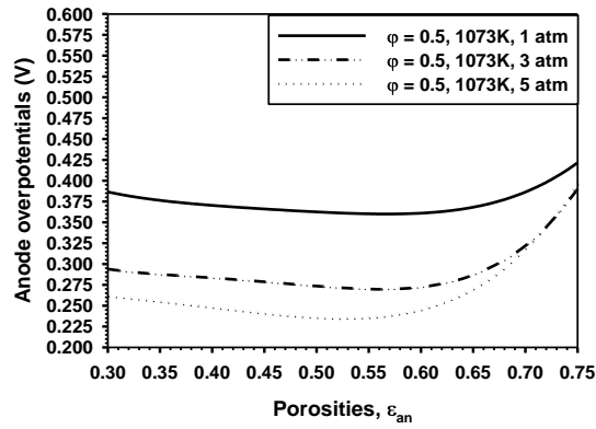
Figure 8. Effect of operating pressure on SOFC overpotentials; (a) corresponding particle radius versus anode overpotentials; (b) porosities versus anode overpotentials.
