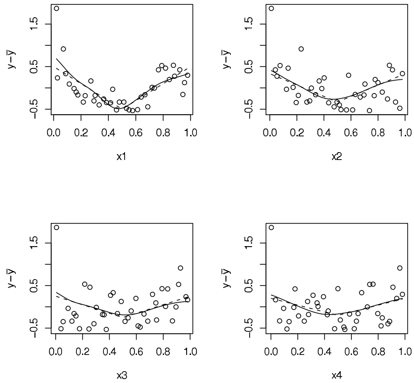
Figure 7: 1-dimensional projections of the observations (bullets) on the g-function example for d = 4 . The univariate models (solid lines) obtained after 5 iterations of RLM are very close to the analytical main effects (dashed lines).
