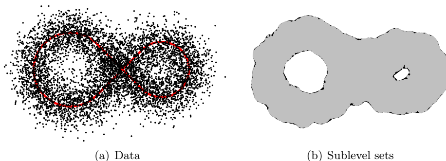
FIGURE 1. (a) 6000 points sampled from a sideways figure 8 (in red), with circle radii R_1 = \sqrt{2} and R_2 = \sqrt{9/8} . The points are sampled from the uniform measure on the figure-8, convolved with the Gaussian distribution \mathcal{N}(0, \sigma^2) where \sigma = .45 . (b) r -sublevel sets of the witnessed (in gray) and exact (additional points in black) k -distances with mass parameter m_0 = 50/6000 , and r = .239 .
