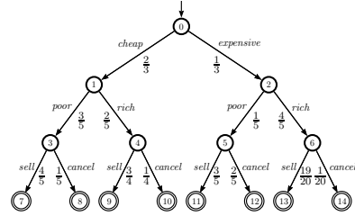
Fig. 4: Ebay Protocol
