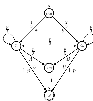
Fig. 1: Crowds Protocol
