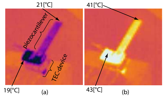
Fig. 11. The thermal images of the piezocantilever using an IR camera.
