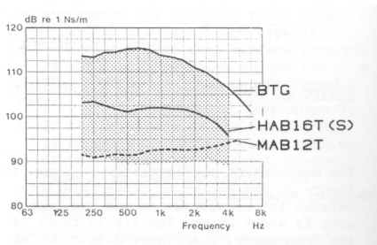
Figure 2.1: Mechanical impedance of road surfaces. Surfaces with high impedance in the high frequency domain [1]
