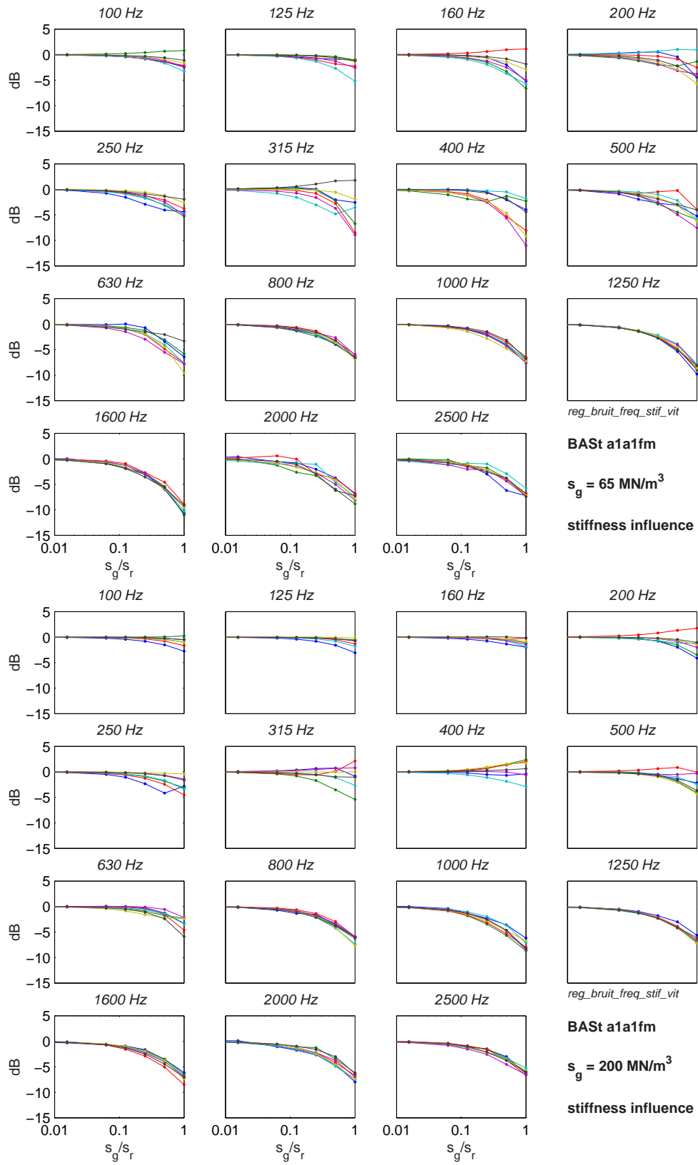
Figure 4.7: \Delta L_W = L_W(v, s_r, f) - L_W(v, \infty, f) as function of s_g/s_r . The noise levels tend to decrease as the road becomes 'softer'
