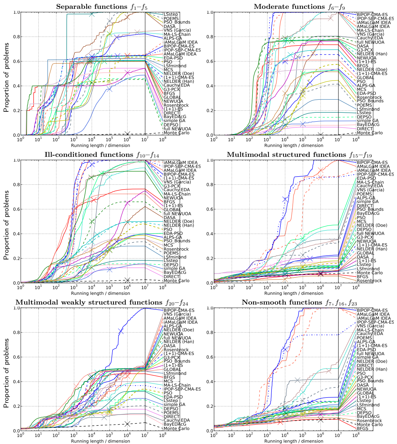
Figure 6: Empirical runtime distributions on function sub-groups with \Delta f_t \in ]100, 10^{-8}] in dimension 20
