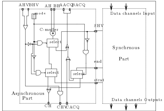
Fig. 4: Elementary processor
