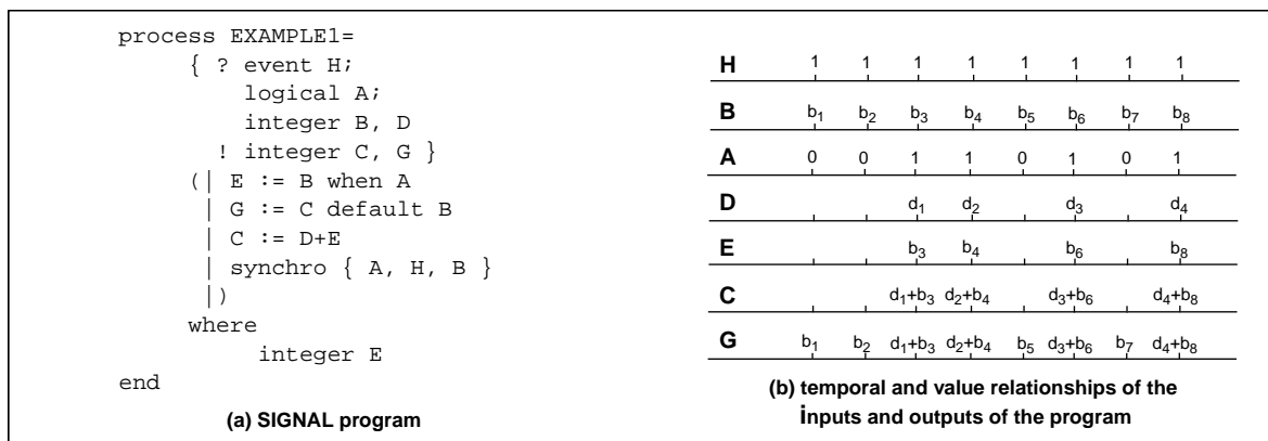
Fig. 1. Functional specification in SIGNAL
