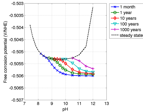
Figure 6.3: Free corrosion potential vs. pH value.
