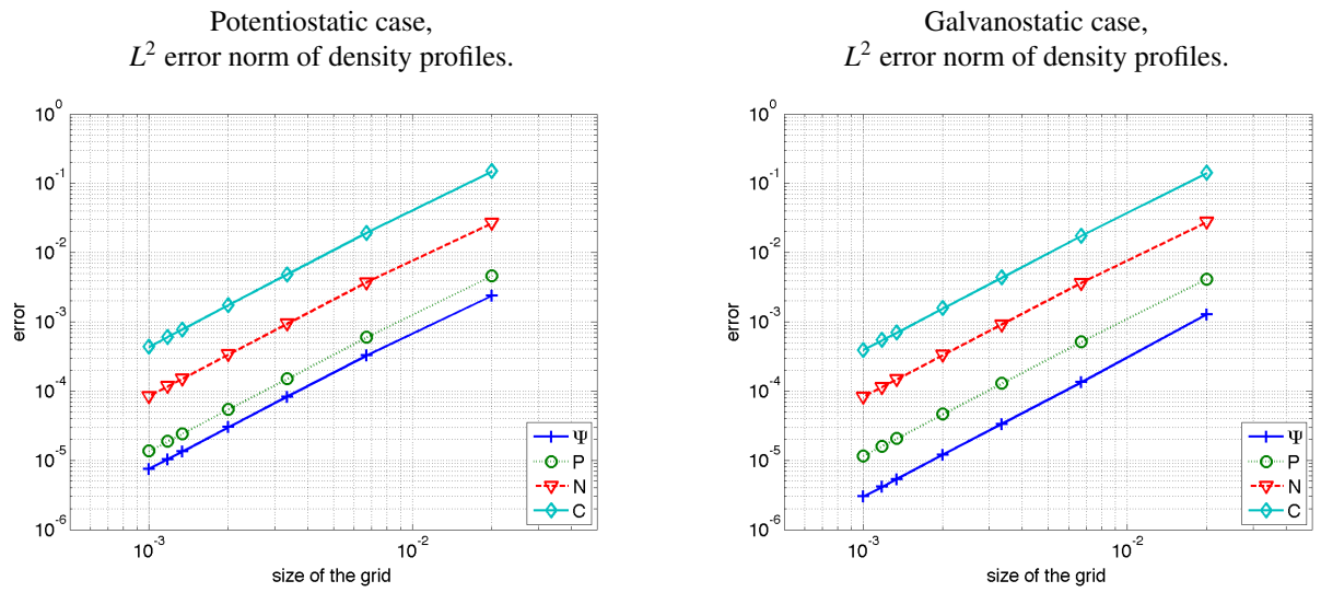
Figure 5.2: Estimated error: difference between the discrete solutions for different grid sizes and a reference solution computed on a grid with 30000 points after 2 h, for \delta = 0.1 and \Delta t_{min} = 5 \cdot 10^{-3} h.
