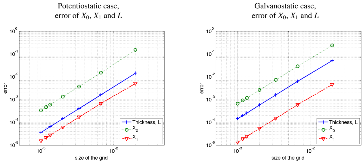
Figure 5.1: Estimated error: difference between the boundary positions for different grid sizes and a those of a reference solution computed on a grid with 30000 points after 2 h, for \delta = 0.1 and \Delta t_{min} = 5 \cdot 10^{-3} h.
