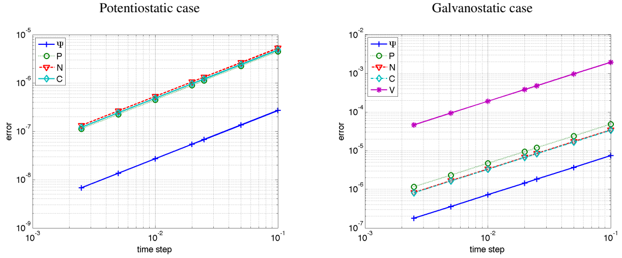
Figure 5.3: Estimated error: difference after 2h between discrete solutions with 2000 grid points for different values of a fixed time step \Delta t and a reference solution computed with \Delta t = 2 \cdot 10^{-6} h.
