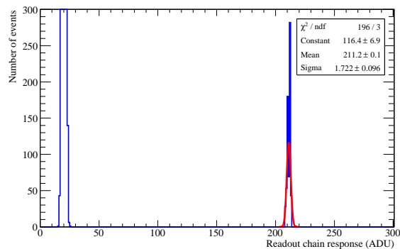
Figure 3: Response of the readout chain to an injected charge of 40 fC.
