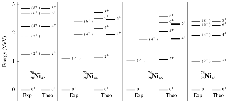
Fig. 2. The low-energy spectra of the nickel isotopes ^{70-76}\text{Ni} . See caption of Fig. 1.
