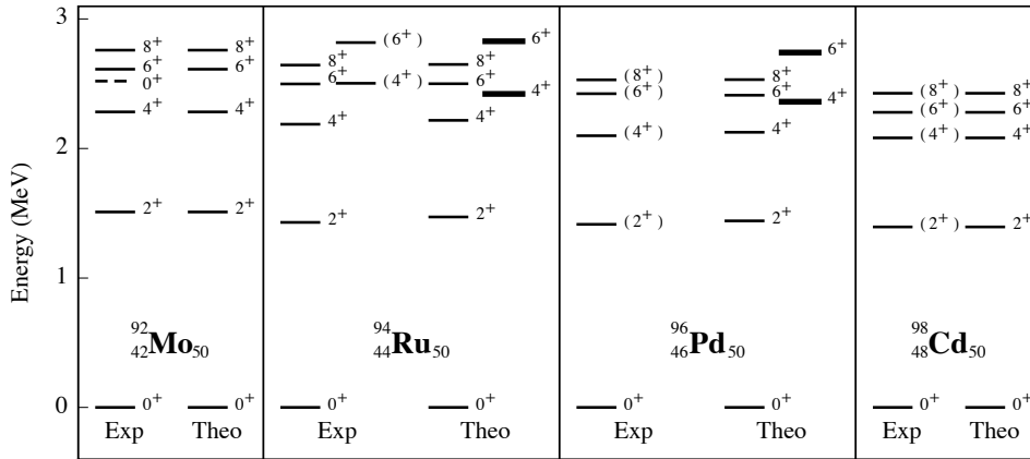
Fig. 1. The low-energy spectra of the N = 50 isotones ^{92}\text{Mo} , ^{94}\text{Ru} , ^{96}\text{Pd} and ^{98}\text{Cd} . The left-hand parts of each panel show the observed levels while the right-hand parts contain the results of a (1g_{9/2})^n shell-model calculation with linearly varying two-body matrix elements. The J^\pi = 4^+ and 6^+ levels with exact v = 4 are shown with thick lines; the dashed line corresponds to an intruder level.
