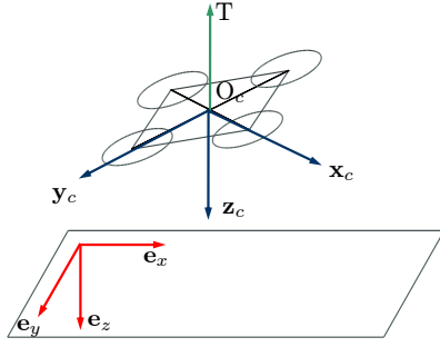
Fig. 4. Frame definitions
