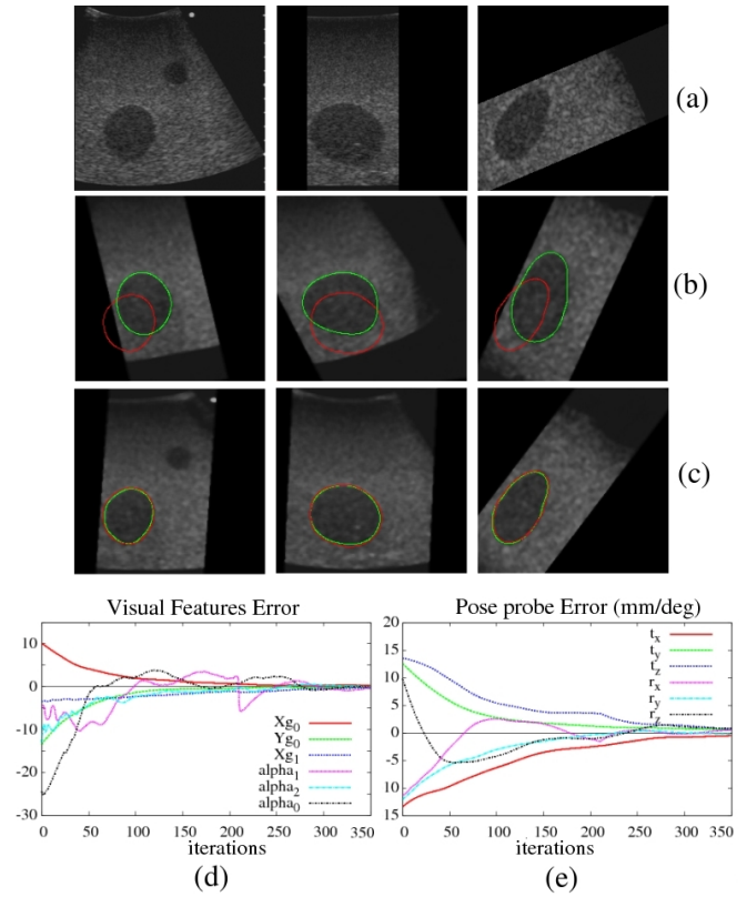
Fig. 5. (a) Intraoperative scan (on left) and interpolated additional orthogonal images (on right). (b), (c) Initial and final images of the virtual probe in the preoperative volume frame. (d), (e) Convergence of the algorithm in term of visual features and pose. A gain \lambda = 0.8 is used in the control law. With an iteration time of 40 \text{ ms} , the registration task is performed in 12 \text{ s} .
