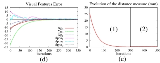
Fig. 6. (a) Intraoperative scan (on left) and interpolated additional orthogonal images (on right). (b), (c) Initial and final preoperative CT images. (d) Evolution of the features error. A gain \lambda = 0.8 is used in the control law and the features convergence is performed in 8 s. (e) Position error of the object section mass center during the visual servoing algorithm (part (1)) and an open loop motion (part (2)).
