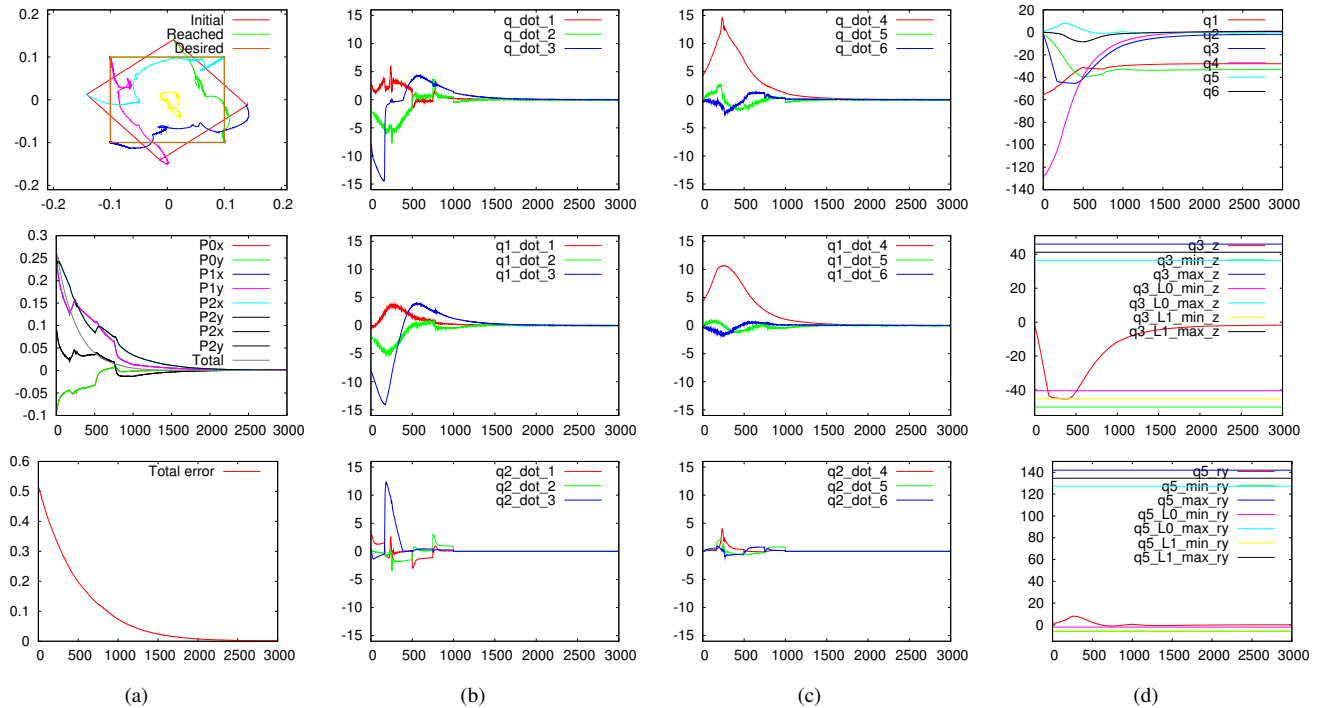
Fig. 4. Results for case 2: Avoidance and additional secondary task sent to translational joints; q2.dot = \dot{\mathbf{q}}_2 + \dot{\mathbf{q}}_3
