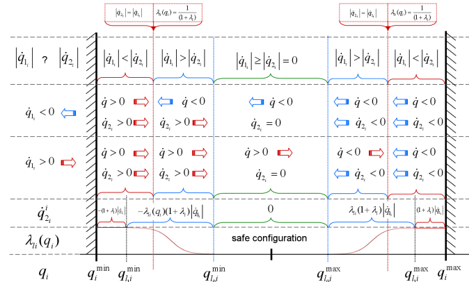
Fig. 2. Comparison between the magnitudes of the i^{th} components \dot{\mathbf{q}}_2^i[i] and \dot{\mathbf{q}}_1[i] where \dot{\mathbf{q}}_2^i[i] is defined by (17) within the different values for q_i of the joint j_i and when \lambda_i > 0 ; Illustration of the relation between the direction of \dot{\mathbf{q}}_1[i] , \dot{\mathbf{q}}_2^i[i] , and \dot{\mathbf{q}}[i] .
