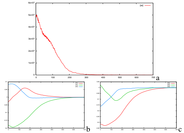
Fig. 7. Stacking luminance and norm of the gradient \mathbf{s} = (\mathbf{I}(\mathbf{r}), \| \nabla \mathbf{I}(\mathbf{r}) \|^2)^\top (a) Cost function, (b) Translational part of \Delta \mathbf{r} (m), (c) Rotational part of \Delta \mathbf{r} (rad.)
