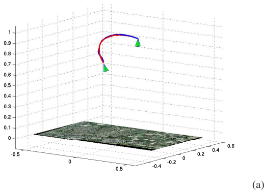
Fig. 9. Reference path of the camera in red and resulting path in blue on the scene in multimodal navigation experiment with initial and final position of the camera. Axis units are in meters.
