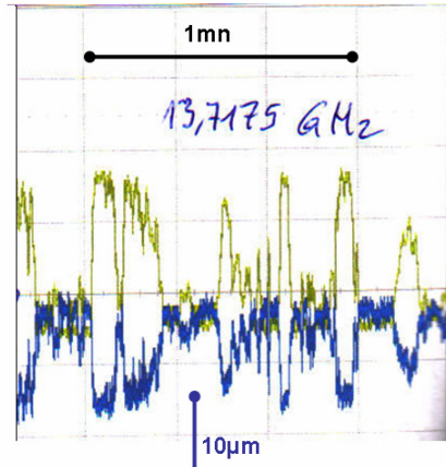
Fig. 5: Typical recording of the open loop telemeter signal (blue trace) and RMS amplitude of the 10MHz-downconverted PHD1 signal (green trace, arb. units)
