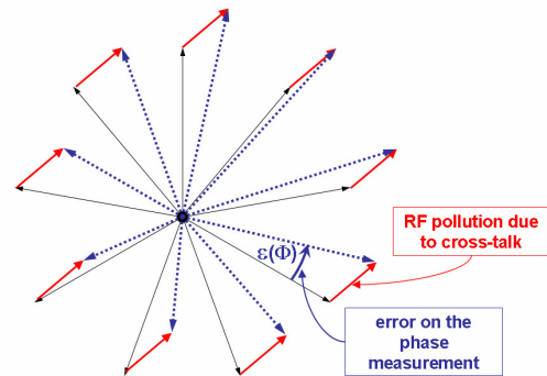
Fig. 1. Amplitude-phase representation showing the cyclic error due to RF cross-talk in a phase measurement.
