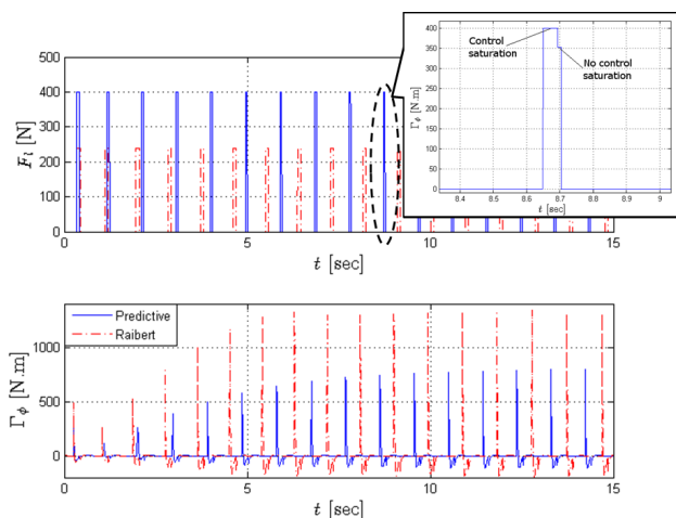
Fig. 7. Evolution of the control inputs versus time
