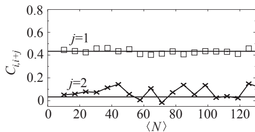
FIG. 6. Correlation of atom number fluctuations between adjacent (open squares) and next-neighbor (crosses) pixels. The solid lines are the predictions for an impulse response function with an rms width of 2.0 \mu\text{m} , obtained by fitting C_{i,i+1} .
