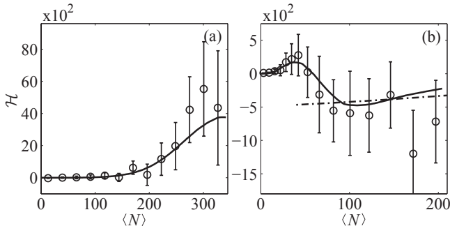
FIG. 3. The measured three-body integral \mathcal{H}_m versus \langle N \rangle , corresponding to the data of Figs. 2 (a) and (b), respectively. The solid (dash-dotted) curves are the thermodynamic predictions from the modified Yang-Yang (quasi-condensate) model.
