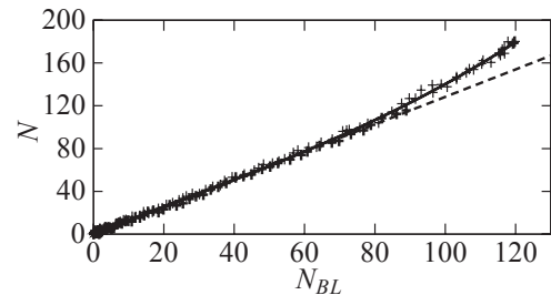
FIG. 5. Experimental determination of the correction to the Beer-Lambert law. The solid curve is a fit to the experimental data with a third-order polynomial, the straight dashed line being the linear contribution. N_{BL} is obtained by using the Beer-Lambert law and summing over transverse pixels in images taken with a nearly resonant probe and a small time of flight of 0.5 ms [see Fig. 4 (a)]. N is obtained from images taken with a probe detuned by 5 MHz and a time of flight of 1.5 ms, for which the Beer-Lambert law is adequate [see Fig. 4 (b)].
