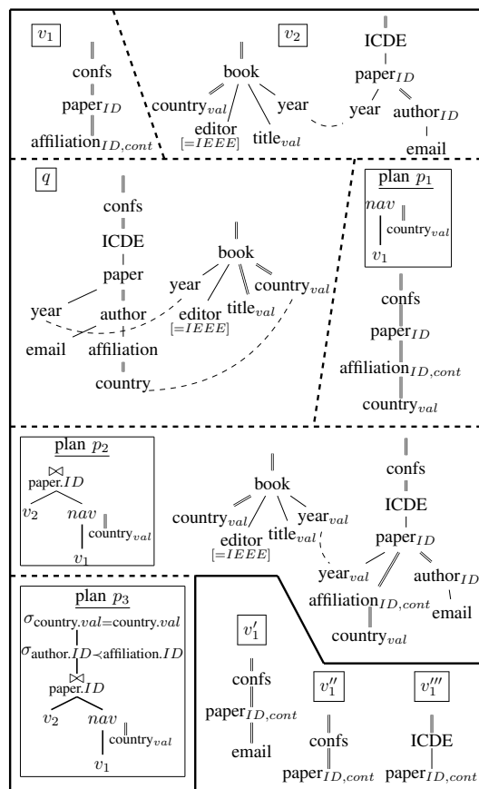
Fig. 1. Sample views, query, and algebraic rewritings.
