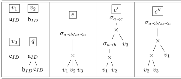
Fig. 5. Sample views, query, non-left-deep rewriting, and two corresponding left-deep rewritings.
