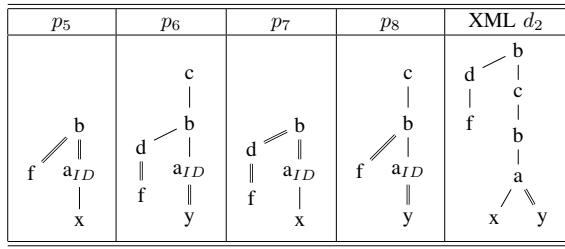
Fig. 7. Zipping XPath queries.
