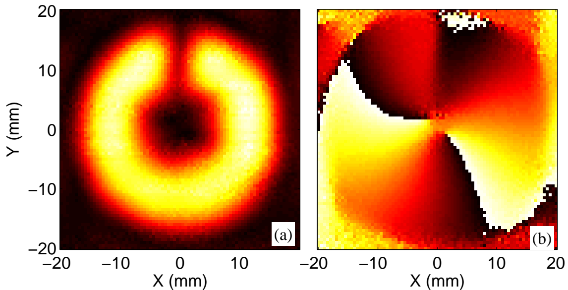
FIG. 12. (Color online) Modulus (a) and phase (b) of vortex of pitch 3 T_0 and duration 1 turn measured at z = 450\text{mm} . The angular frequency is located between two spectral lines of Fig. 4 at 2.5/3\omega_0
