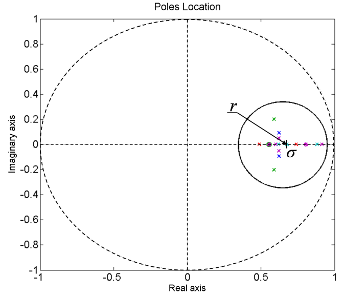
Fig. 6. Pole placement region.
