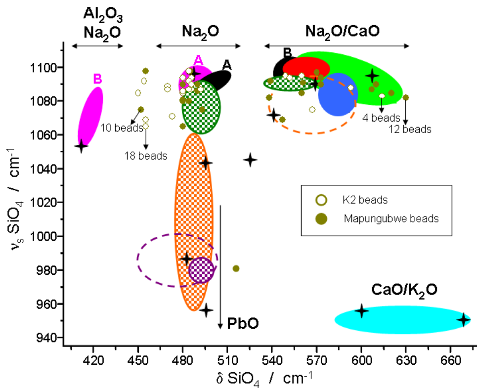
Figure 10: Classification using the SiO 4 bending massive versus stretching massive plot a) of a large glass corpus (1, Ricciardi et al., 2009b; 2, Kirmizi et al., 2010a; 3, Kirmizi et al., 2010b; 4, Colomban et al., 2006a; 5, Tournié, 2009) and b) plus the data of the beads excavated at Mapungubwe hill and K2.
