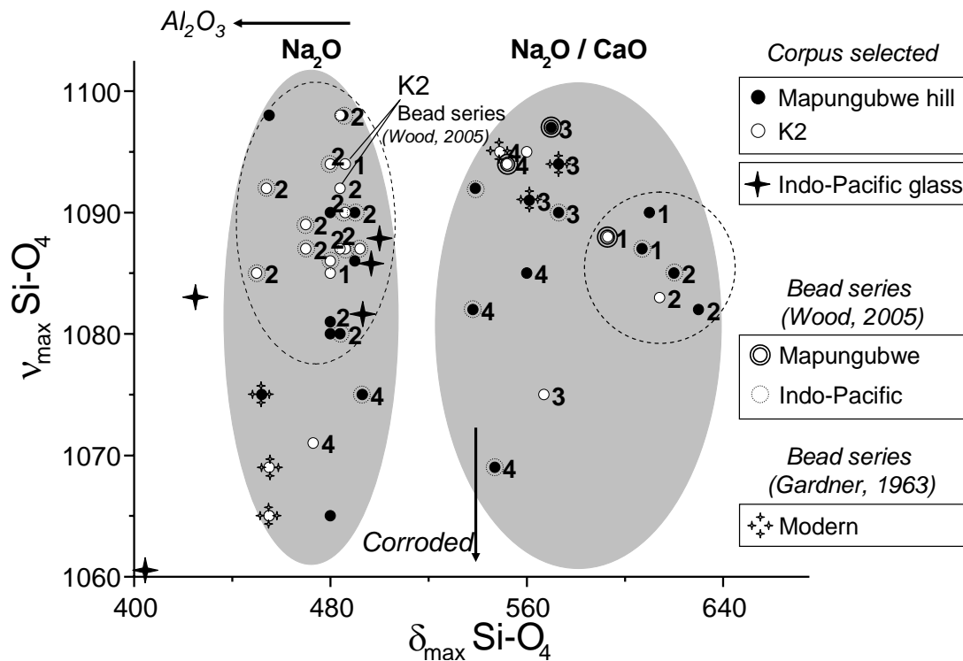
Figure 12: Classification of the glass beads from Mapungubwe hill and K2 sites according to the bending and stretching massive of \text{SiO}_4 . The type of glass matrix ( \text{Na}_2\text{O} and \text{Na}_2\text{O}/\text{CaO} ), the tendency of glass matrix ( \text{Al}_2\text{O}_3 , \text{PbO} or corroded) and the bead series (K2, Mapungubwe, Indo-Pacific and European) are also indicated.
