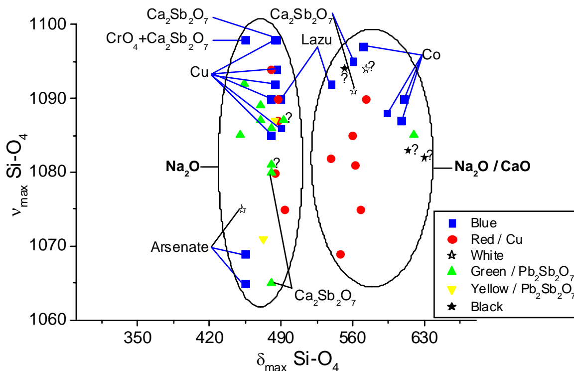
Figure 12: Classification of the glass beads from Mapungubwe hill and K2 sites. The colours and pigments of the beads are indicated.
