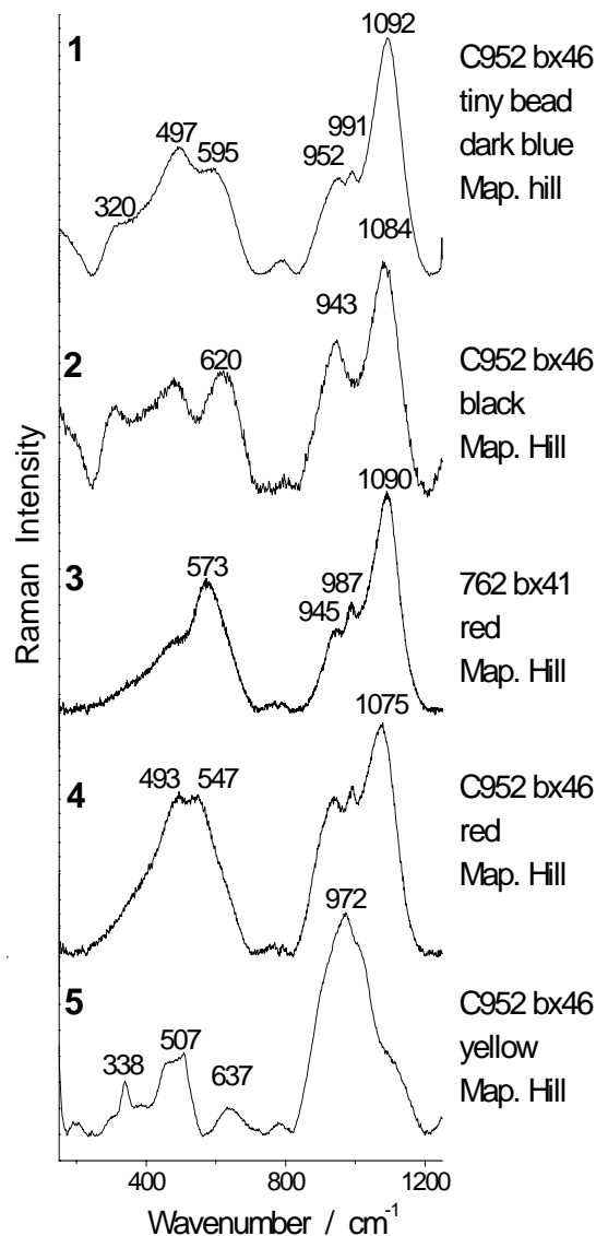
Figure 11: Representative Raman signatures of the five types glass matrix observed among the corpus of glass beads. The type 2 is a soda glass. The type 3 is soda-lime glass, the type 4 is a corroded glass and the type 5 corresponds to the lead. The type 1 seems to be an intermediate between the type 2 and 3.
