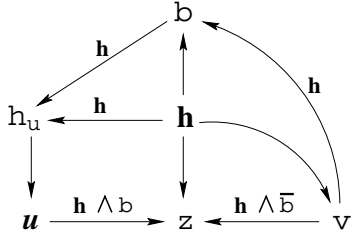
Figure 1: Scheduling from causality analysis for the example.
