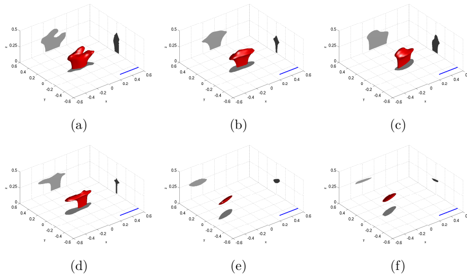
FIGURE 6.4. Experiment 2: Reconstructions of the submarine from limited aperture data (1/8 horizontal aperture). Blue lines in the plots indicates the wave length. (a) Conjugate incident point sources, no noise. (b) Conjugate incident point sources, 1% relative noise. (c) Conjugate incident point sources, 5% relative noise. (d) Physical incident point sources, no noise. (e) Physical incident point sources, 1% relative noise. (f) Physical incident point sources, 5% relative noise.
