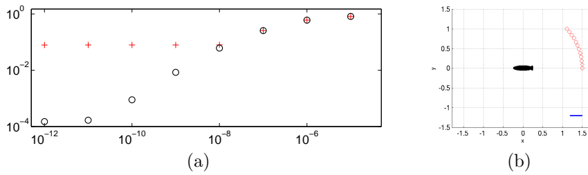
FIGURE 6.3. (a) The error \|N_{\text{phys}}P_{\delta} - N\|/\|N\| versus \delta , in the setting used for the reconstructions shown in Figure 6.2. Norms of matrices are measured in the spectral norm. Circles (o) correspond to errors computed without adding artificial noise to N and N_{\text{phys}} . Pluses (+) correspond to errors computed from noisy versions of N and N_{\text{phys}} at a noise level of 5%. (b) Horizontal positions of the sources (red circles) for experiment 2.
