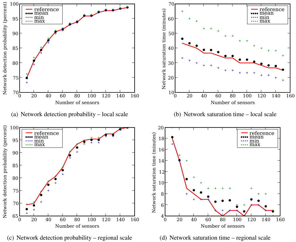
Figure 11: Influence of wind speed variations: evolution of the mean detection probability and saturation time with a wind speed variation between -35\% and +35\% , at local and regional scale. Reference is the situation 1. Networks are defined with the sensors having the highest detection probability.
