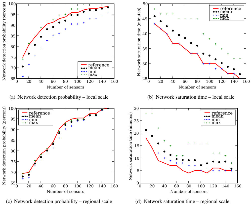
Figure 12: Influence of wind angle variations: variations of detection probability and saturation time with a wind speed variation between -25^\circ and +25^\circ at local and regional scale. Reference is the situation 1. Networks are defined with the sensors having the highest detection probability.
