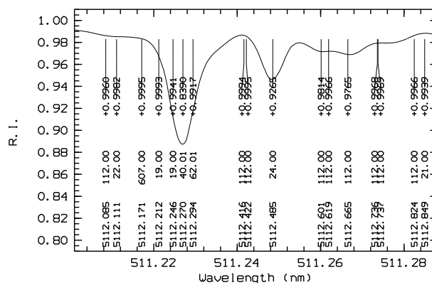
Fig. 12 The observed solar disc-centre spectrum of Delbouille et al. (1973) in the region of the Zr II line at 511.2 nm (black solid) with the identifications of the lines in the range according to the line list of Kurucz.
