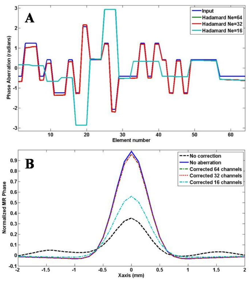
Figure 15 a) Recovered phase aberration profiles from simulated experiments: input, recovered with 64, 32 and 16 independent channels. b) Recovered spatial profiles of the simulated MR phase without any correction, with no aberration, with corrected phase profiles obtained from the full 4*64 emissions acquisition and from the decimated acquisition to 32 or 16 independent channels.
