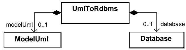
Figure 3- Metamodel used to check the constraints with OCL
