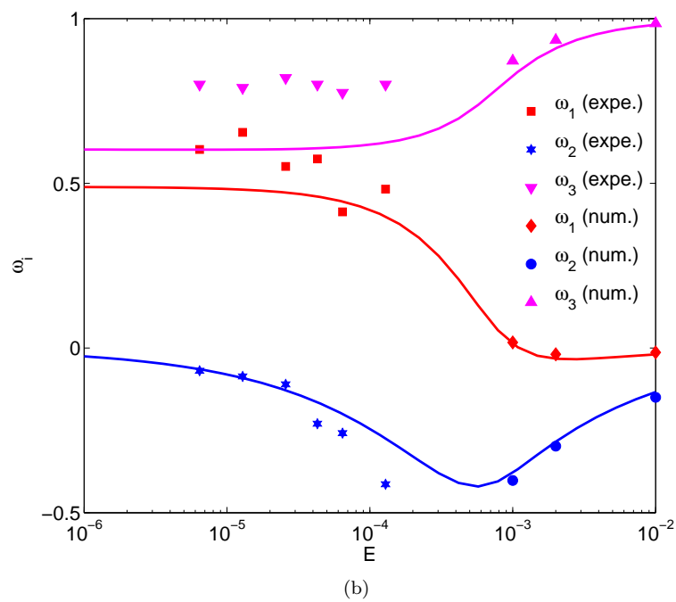
FIG. 3: Comparison of the theoretical rotation rate components of Busse's solution for a spheroid (continuous lines) with experimental PIV measurements and numerical simulations performed over a large range of Ekman numbers for \Omega_p = -0.14 and a_3/a_1 = 0.85 . (a) For a precession angle of 5^\circ . (b) For a precession angle of 15^\circ .
