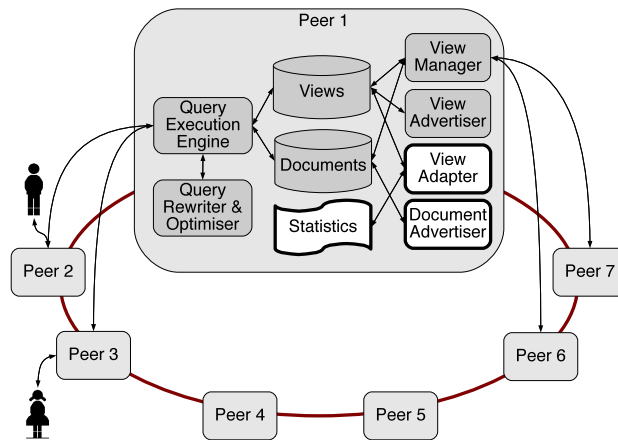
Figure 1: LiquidXML platform architecture.
