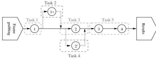
Figure 7 Split of a vision processing chain into tasks, using Cléopatre's DM and IC.
