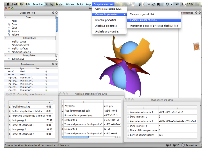
Fig. 5. GENOM3CK on the input curve defined by F(x, y) = x^2 - y^5
