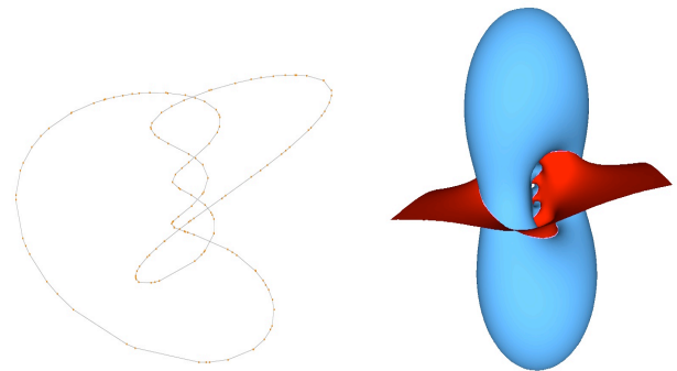
(a) Algebraic link of (0, 0)
