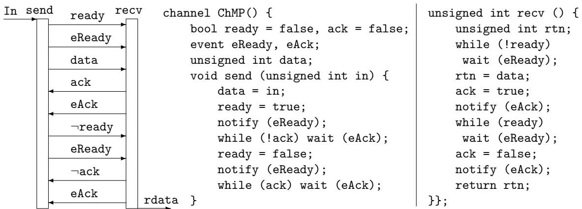
Figure 29. Implementation of a channel with double hand-shake in SPECC.
