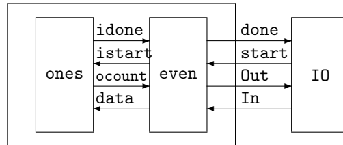
Figure 26. Functional architecture of an even-parity checker (EPC).
