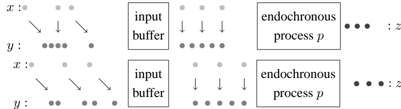
Figure 11. Endochrony: from flow-equivalent inputs to clock-equivalent outputs
