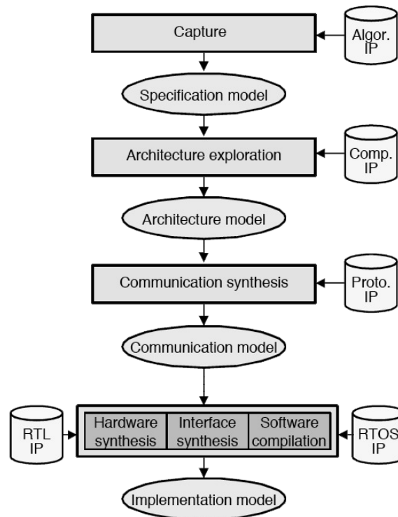
Figure 18. SPECC design methodology [15]
