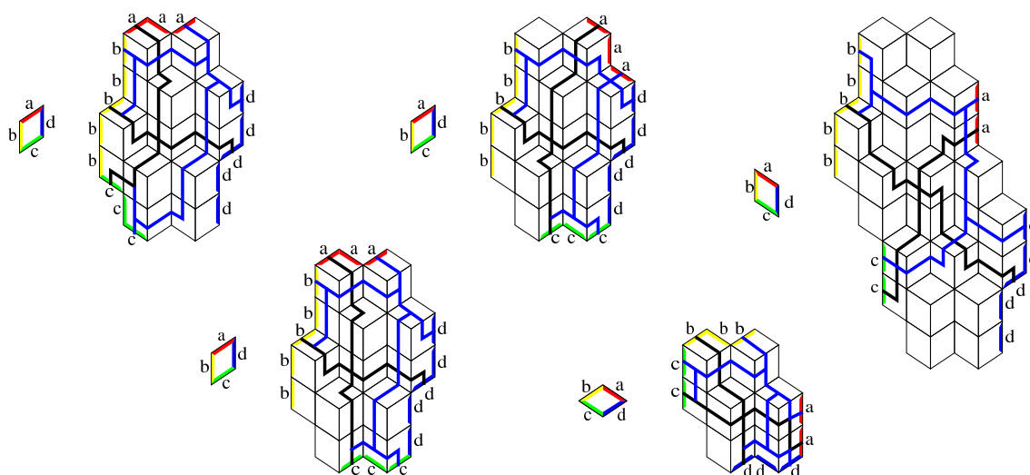
Figure 6: A second network for the Rauzy combinatorial substitution.
