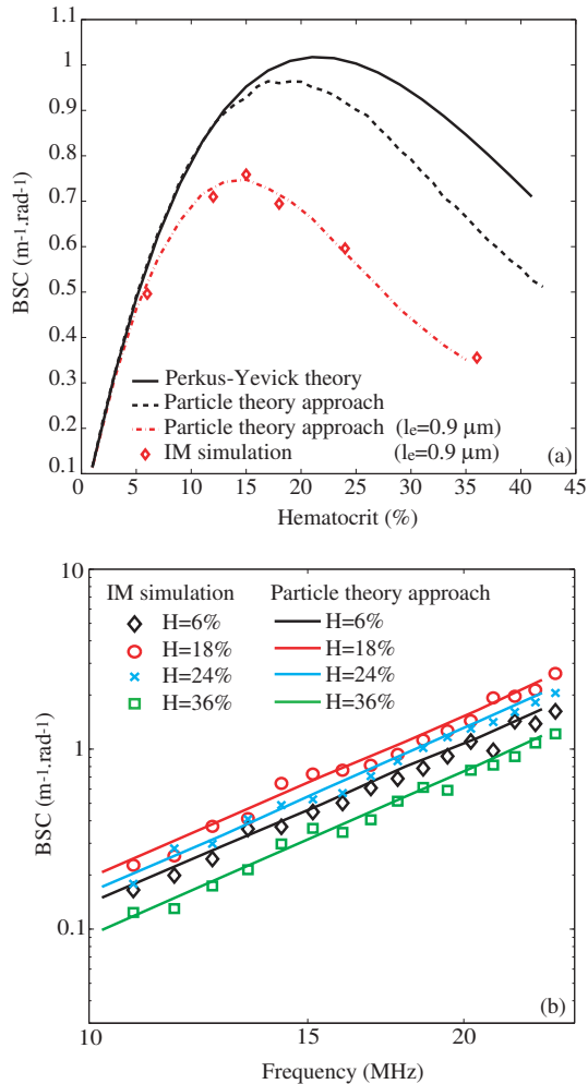
FIGURE 3 – (a) Plots of backscatter coefficients versus the hematocrit for non-aggregated RBCs. The solid curve represents the BSC_{theo} calculated with the Percus-Yeivick packing factor, the dashed lines the particle theory approach BSC_{theo} obtained by computing the structure factor with and without the exclusion length. The diamond markers express simulation results BSC_{sim} . (b) Frequency-dependent backscattering coefficients for an hematocrit of 6, 18, 24 and 36% in the case of non-aggregated RBCs. The solid line represents the curve for the particle theory approach. Simulations results are shown by the symbols.
