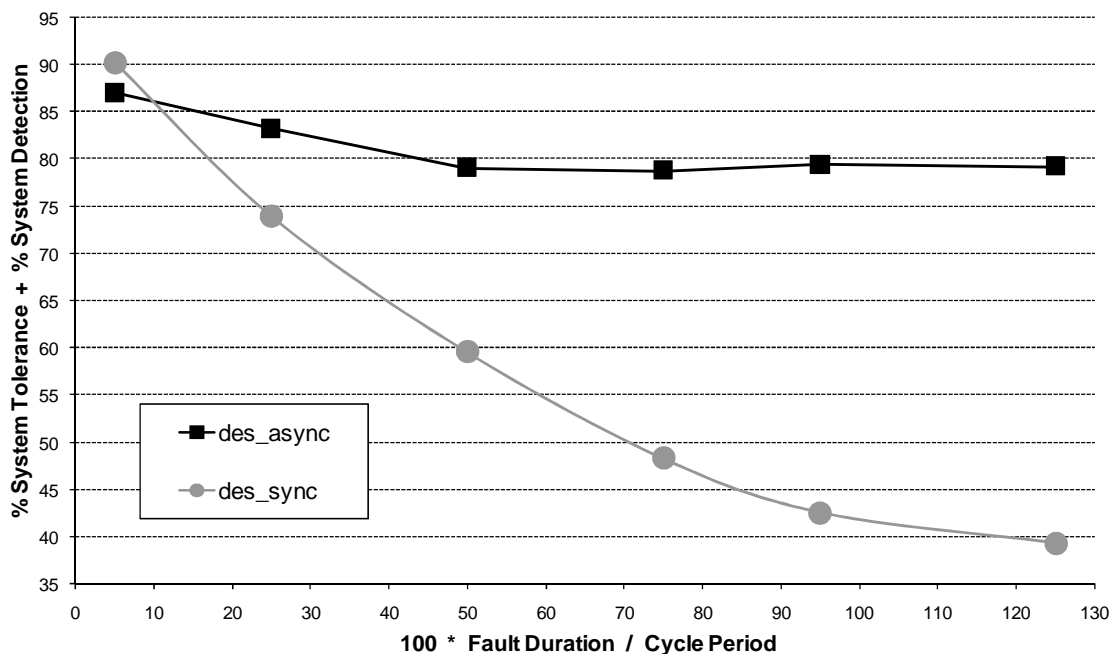
Figure 5.3: The stronger natural ability of a QDI asynchronous system for mitigation of LDT faults in deep-submicron technologies
