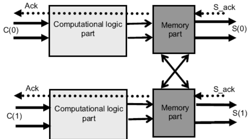
Figure 6.6: Synchronization Technique for two bits of a data word in a QDI system (MONNET, 2005-b)
