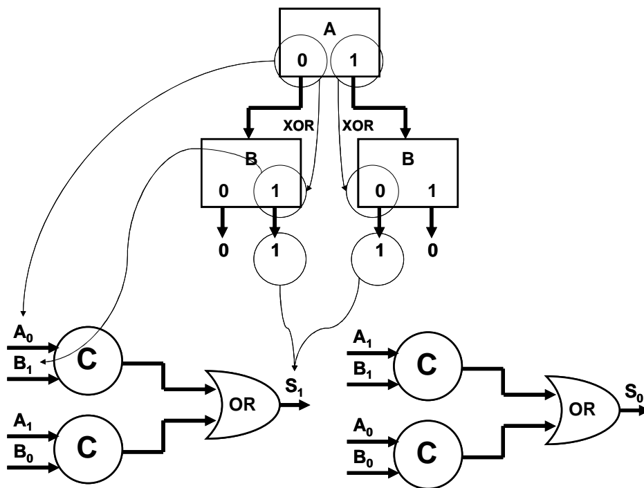
Figure 2.7: MDD-based logic synthesis of a delay-insensitive dual-rail XOR function for the four-phase protocol
