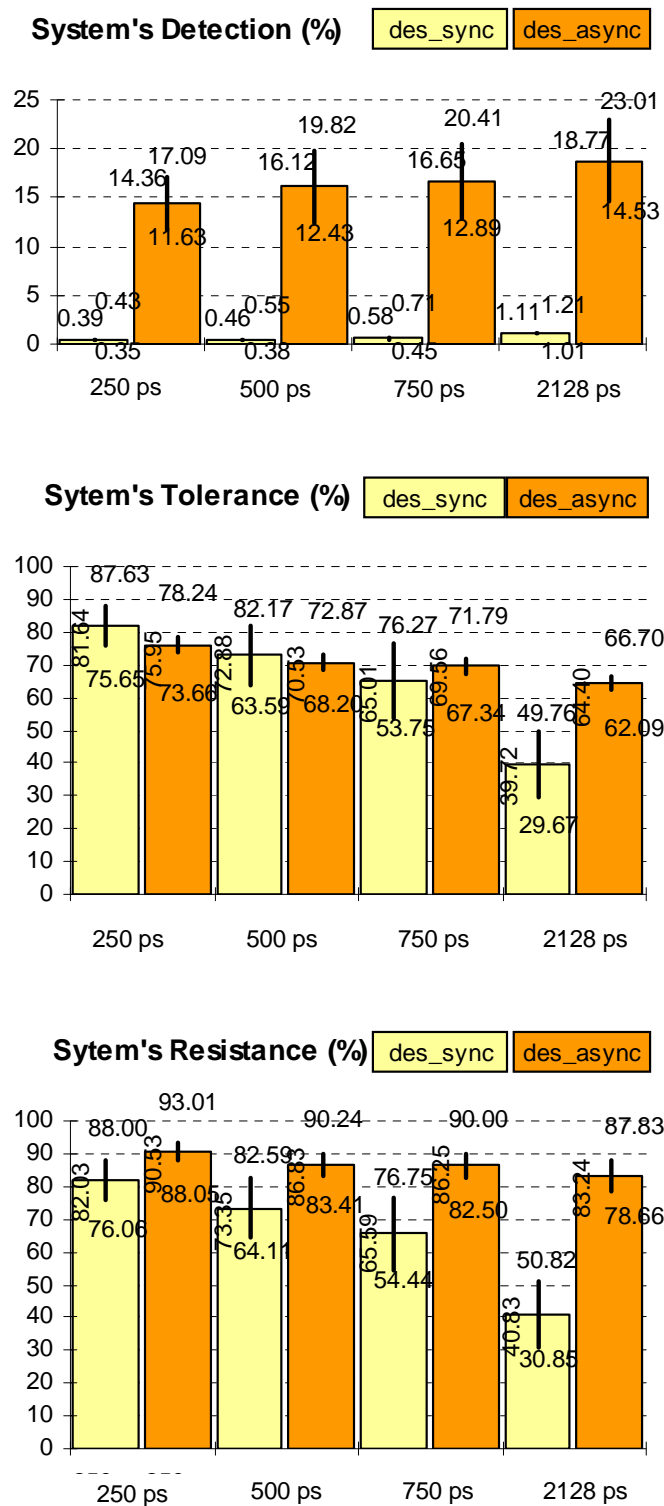
Figure 4.10: System-robustness percentages
