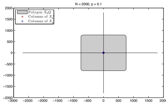
Fig. 7. Shape of the polytope \bar{X}_k Q , K = 3 , p = 0.1 and N = 2000 . The data was drawn according to the Bernoulli-Gaussian model described in Section V, and is highly sparse. The shape is close to a cube.
