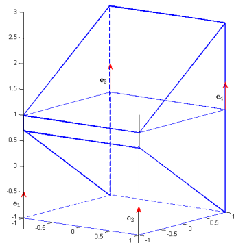
Figure 5: Examples of admissible hexahedra
