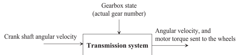
Figure 3. Transmission block
