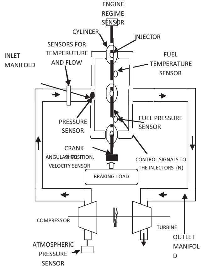
Figure 2. Engine Architecture, [10]
