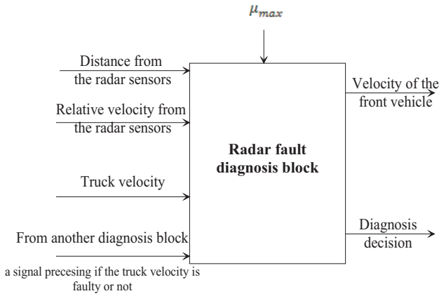
Figure 6. Radar fault diagnosis block
