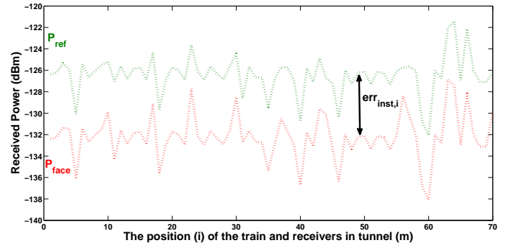
Fig. 5. The computation of the gap between P_{ref} and P_{face}
