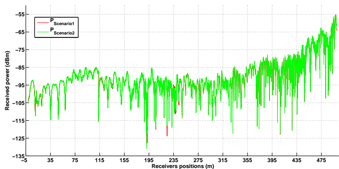
Fig. 9. Evolution of total received power for different environments modeling
