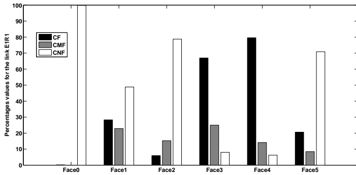
Fig. 6. Identification of contributory faces , medium contributory faces and non-contributory faces for the SISO link E1R1
