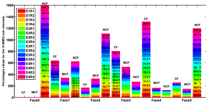
Fig. 7. Identification of contributory faces , medium contributory faces and non-contributory faces for the 16 MIMO sub-channels
