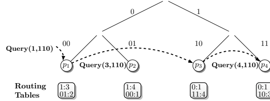
Figure 5: Example of P-Grid binary tree.
