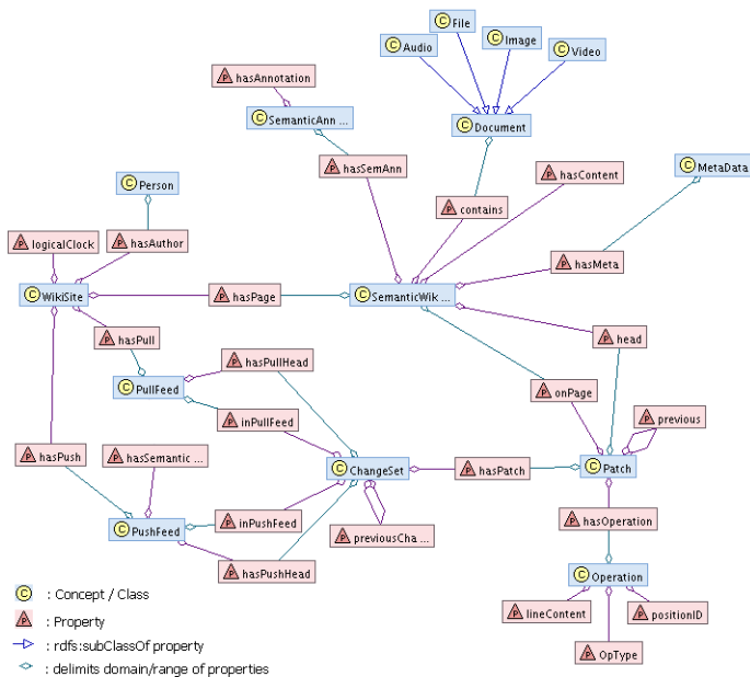
Fig. 1. Multi-synchronous ontology
