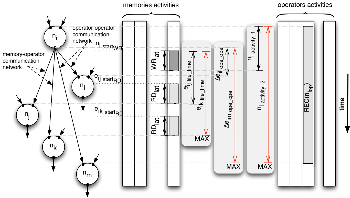
Fig. 5. Example with communications on both networks.
